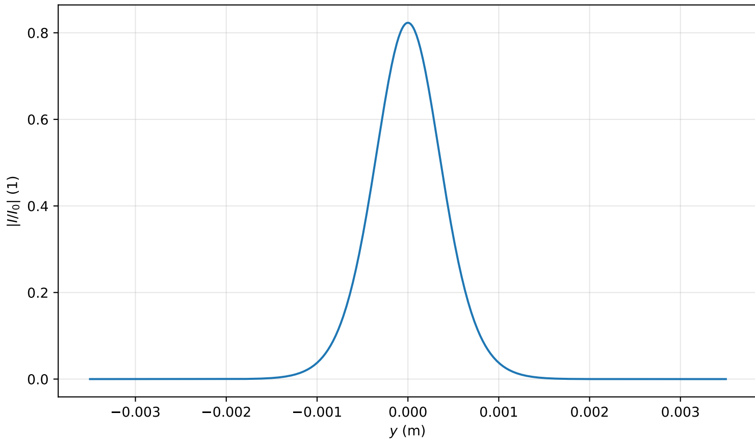
Intensity profile I(x=0, y, z=1.672)/I_0 , \text{Pin}=0.4\text{Pcr} , artificial time
